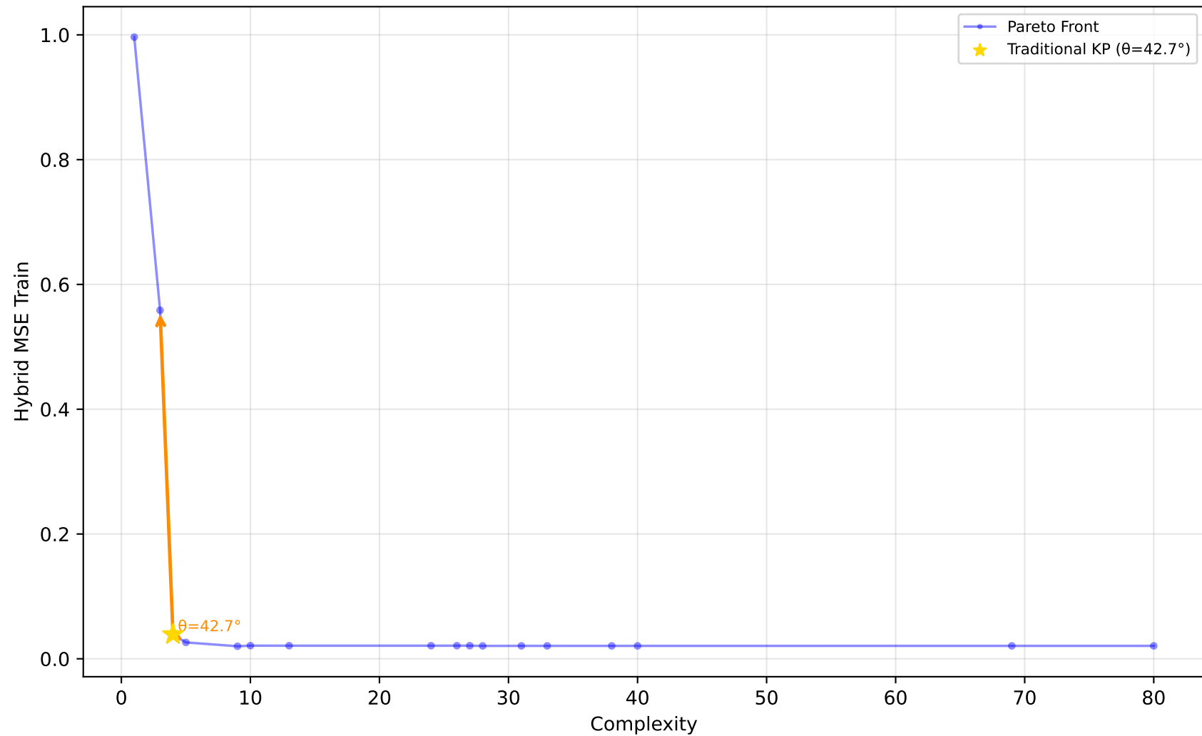
523_analcatdata_neavote - Run 10 - MVP - Hybrid MSE Train \lambda_1=0.00, \lambda_2=0.10, \lambda_3=0.00 | Difficulty: 1.00 | Method: hmr
