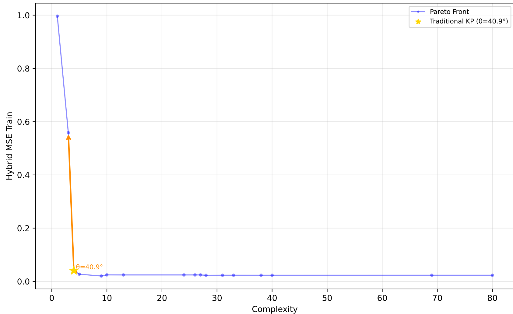
523_analcatdata_neavote - Run 10 - MVP - Hybrid MSE Train \lambda_1=0.00, \lambda_2=0.40, \lambda_3=0.00 | Difficulty: 1.00 | Method: hmr
