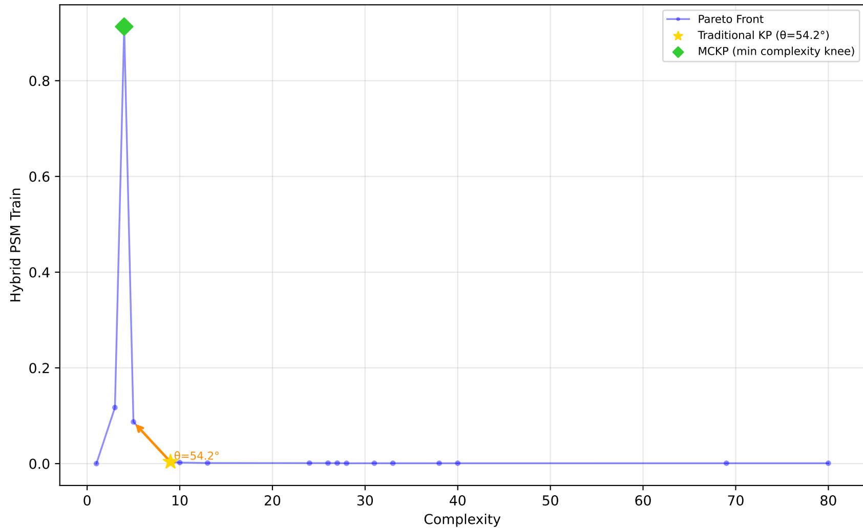
523_analcatdata_neavote - Run 10 - MVP - Hybrid PSM Train \lambda_1=0.00, \lambda_2=0.10, \lambda_3=0.00 | Difficulty: 1.00 | Method: hmr
