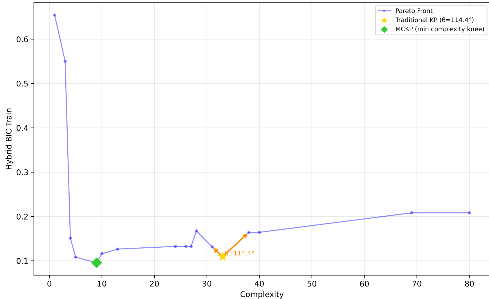
523_analcatdata_neavote - Run 10 - SVP - Hybrid BIC Train \lambda_1=0.00, \lambda_2=0.90, \lambda_3=0.00 | Difficulty: 1.00 | Method: hmr
