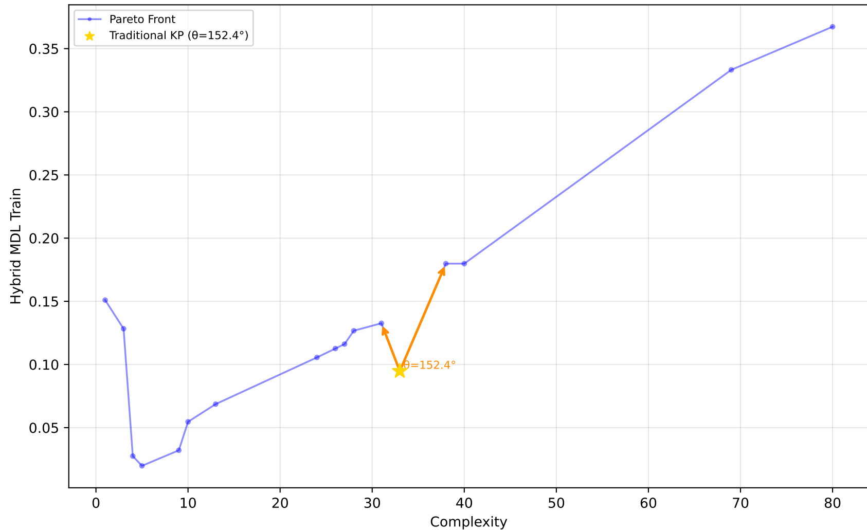
523_analcatdata_neavote - Run 10 - SVP - Hybrid MDL Train \lambda_1=0.00 , \lambda_2=0.20 , \lambda_3=0.00 | Difficulty: 1.00 | Method: hmr
