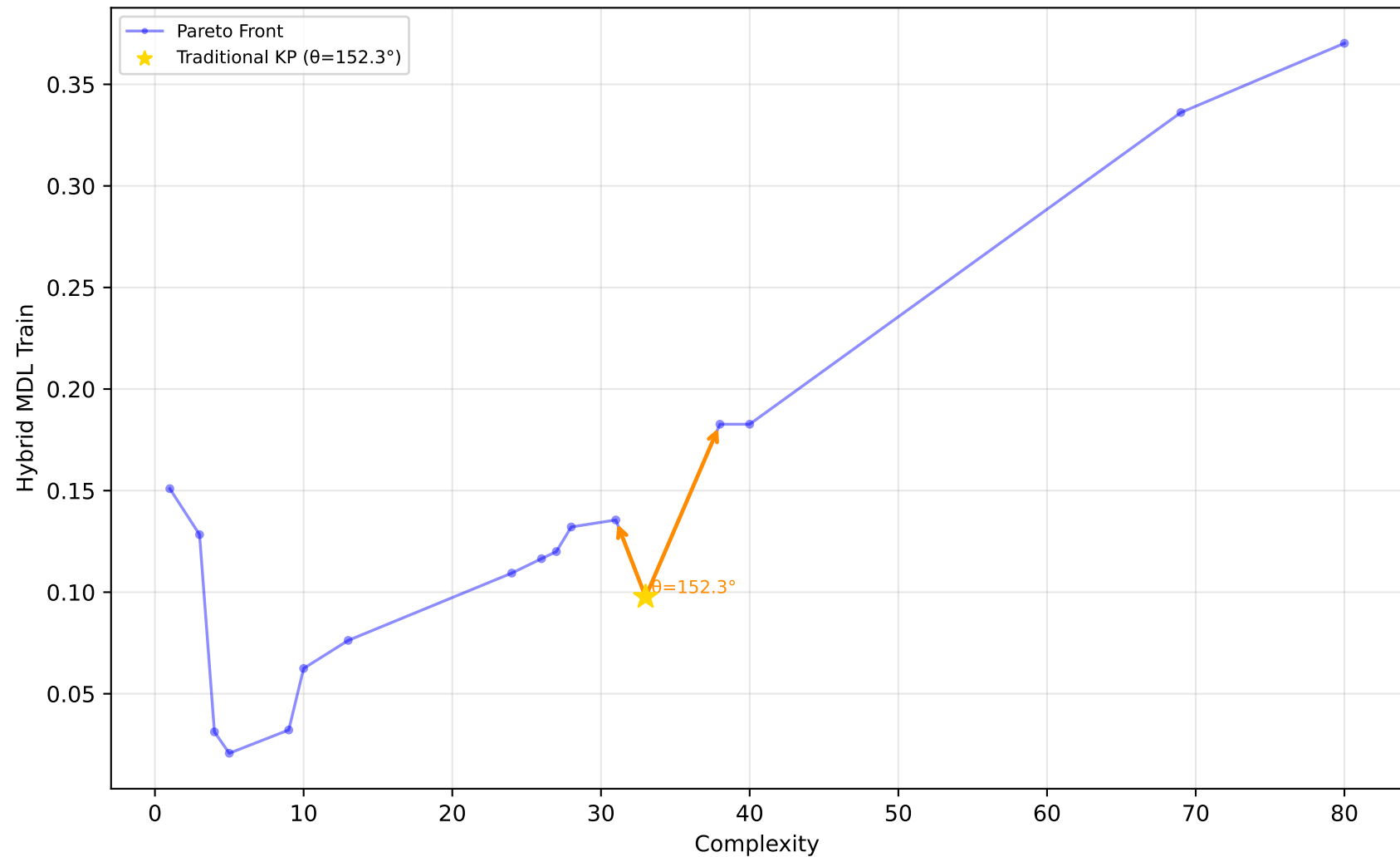
523_analcatdata_neavote - Run 10 - SVP - Hybrid MDL Train \lambda_1=0.00, \lambda_2=0.90, \lambda_3=0.00 | Difficulty: 1.00 | Method: hmr
