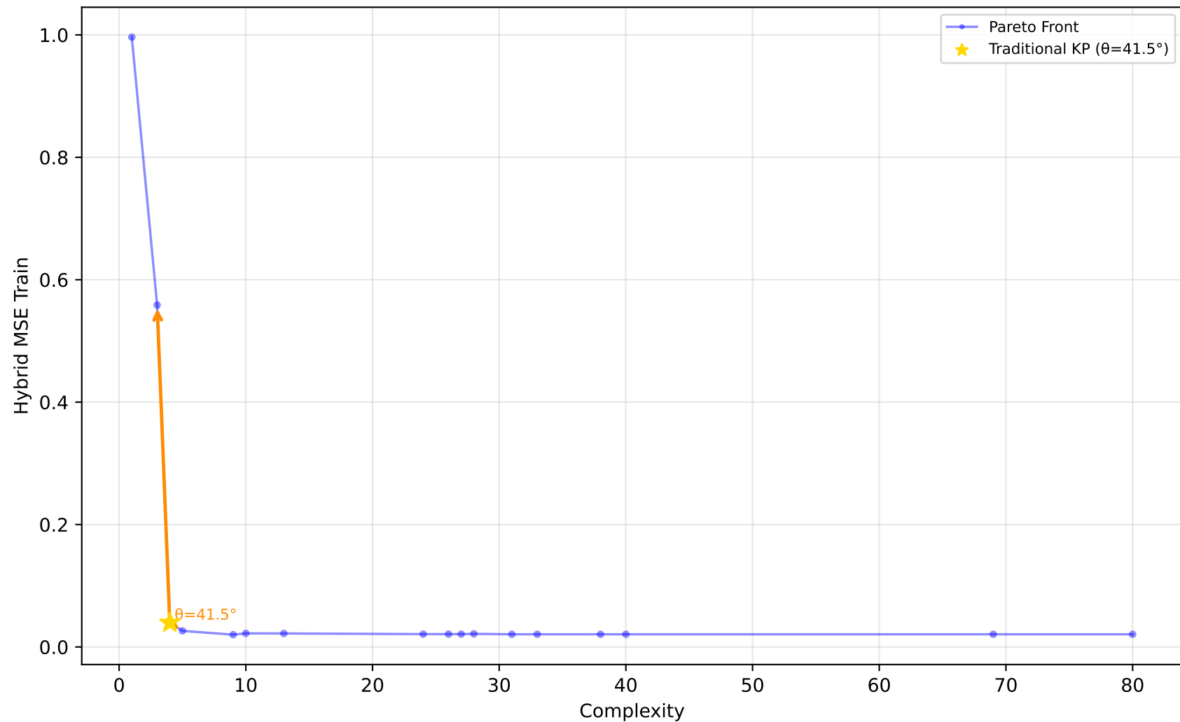
523_analcatdata_neavote - Run 10 - SVP - Hybrid MSE Train \lambda_1=0.00, \lambda_2=0.20, \lambda_3=0.00 | Difficulty: 1.00 | Method: hmr
