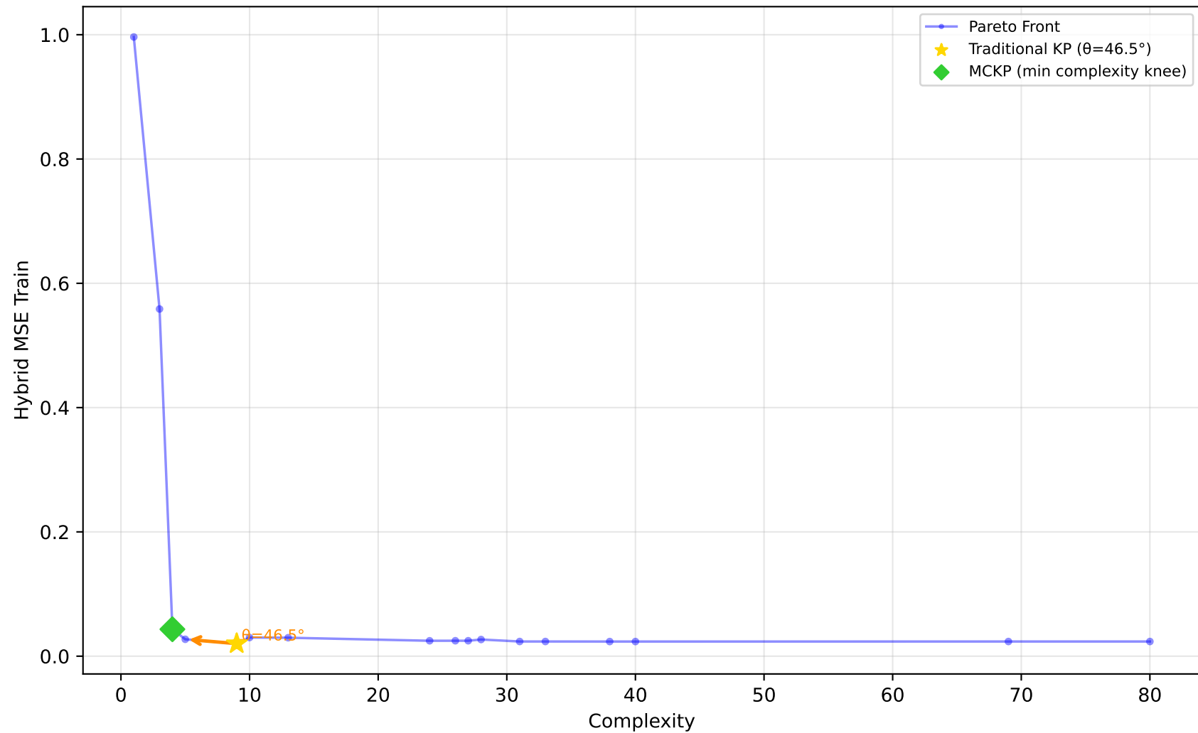
523_analcatdata_neavote - Run 10 - SVP - Hybrid MSE Train \lambda_1=0.00, \lambda_2=0.90, \lambda_3=0.00 | Difficulty: 1.00 | Method: hmr
