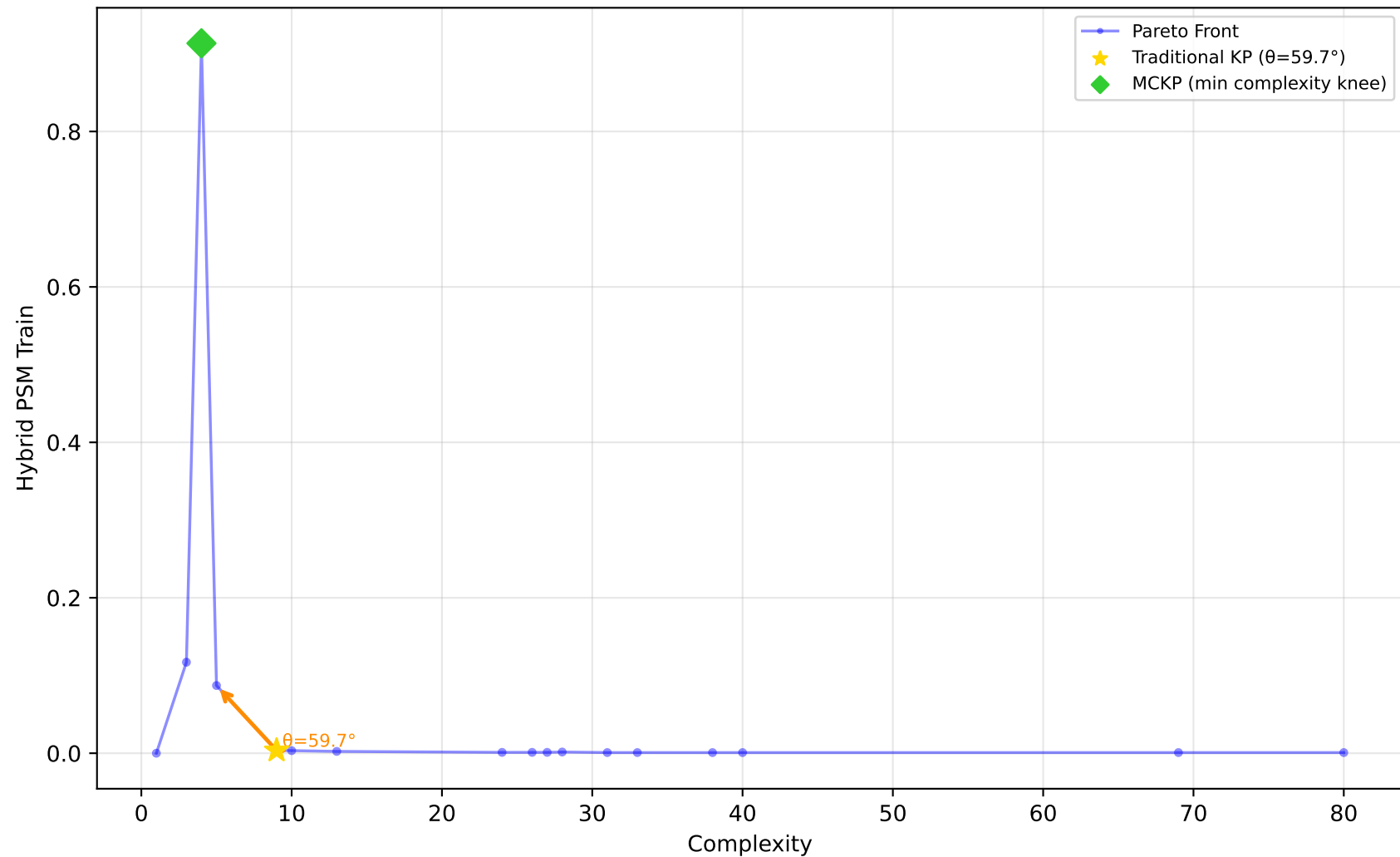
523_analcatdata_neavote - Run 10 - SVP - Hybrid PSM Train \lambda_1=0.00 , \lambda_2=0.20 , \lambda_3=0.00 | Difficulty: 1.00 | Method: hmr
