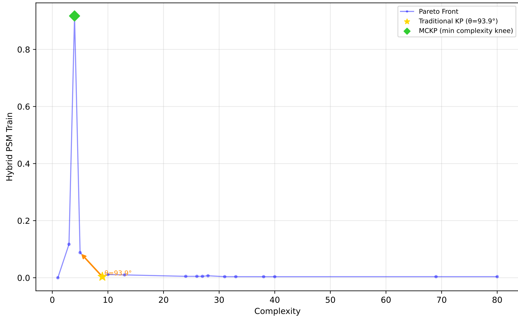
523_analcatdata_neavote - Run 10 - SVP - Hybrid PSM Train \lambda_1=0.00, \lambda_2=0.90, \lambda_3=0.00 | Difficulty: 1.00 | Method: hmr
