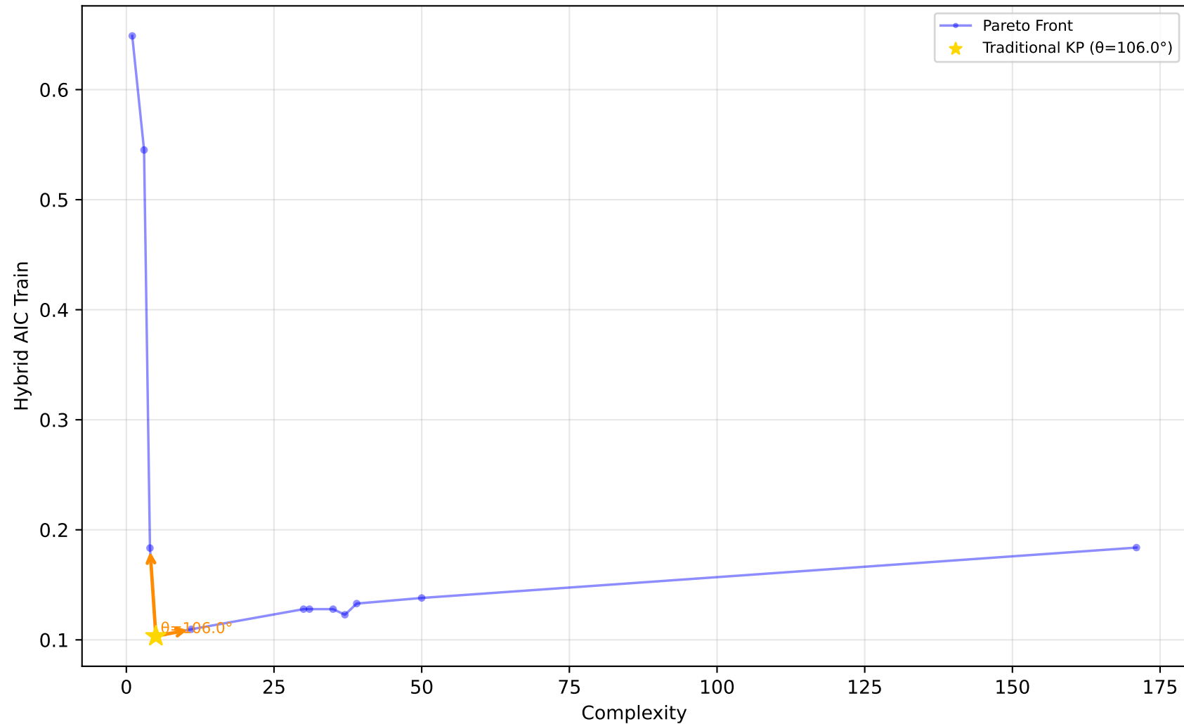
523_analcatdata_neavote - Run 11 - MVP - Hybrid AIC Train \lambda_1=0.00, \lambda_2=0.10, \lambda_3=0.00 | Difficulty: 1.00 | Method: hmr
