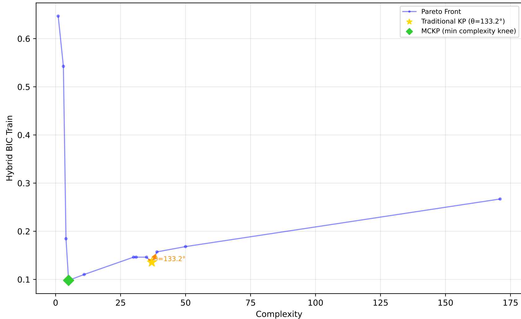
523_analcatdata_neavote - Run 11 - MVP - Hybrid BIC Train \lambda_1=0.00, \lambda_2=0.10, \lambda_3=0.00 | Difficulty: 1.00 | Method: hmr
