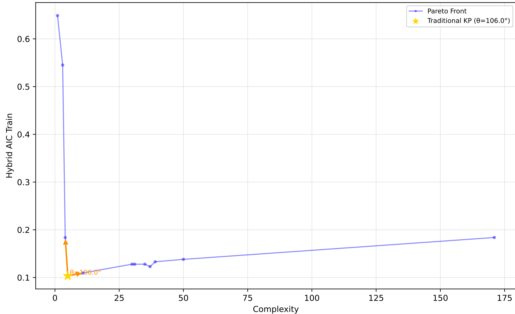
523_analcatdata_neavote - Run 11 - SVP - Hybrid AIC Train \lambda_1=0.00 , \lambda_2=0.20 , \lambda_3=0.00 | Difficulty: 1.00 | Method: hmr
