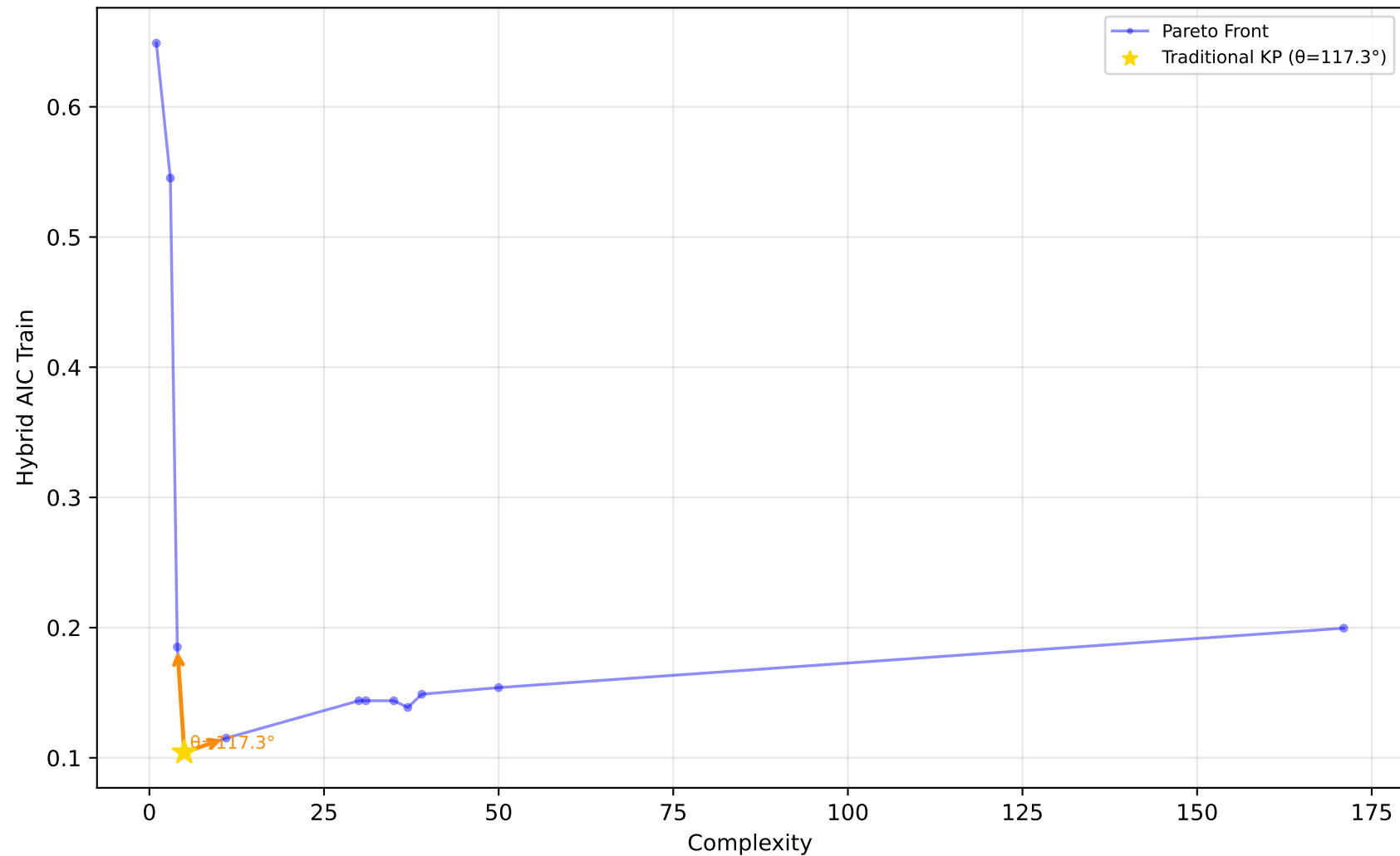
523_analcatdata_neavote - Run 11 - SVP - Hybrid AIC Train \lambda_1=0.00, \lambda_2=0.90, \lambda_3=0.00 | Difficulty: 1.00 | Method: hmr
