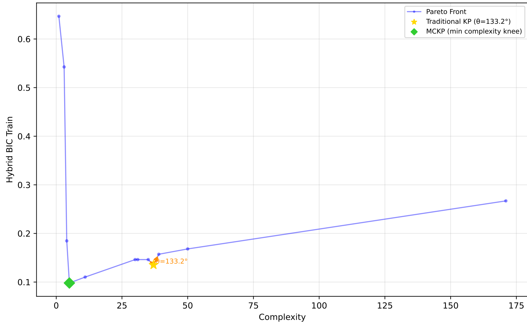
523_analcatdata_neavote - Run 11 - SVP - Hybrid BIC Train \lambda_1=0.00 , \lambda_2=0.20 , \lambda_3=0.00 | Difficulty: 1.00 | Method: hmr
