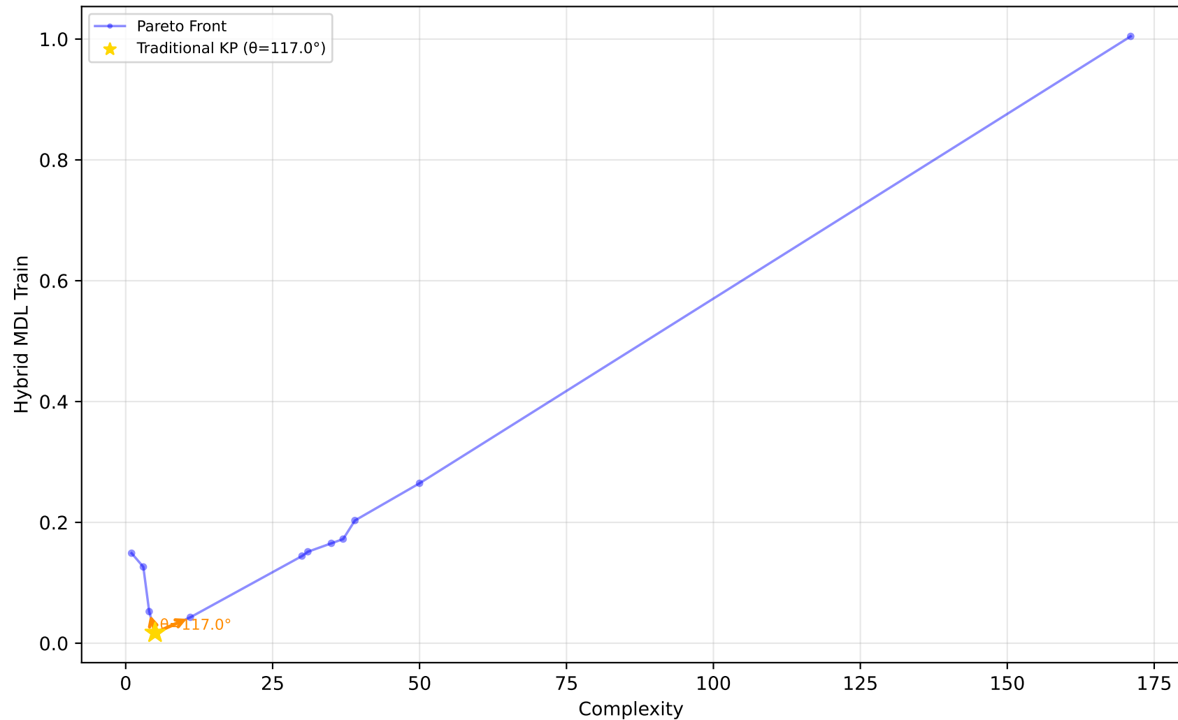
523_analcatdata_neavote - Run 11 - SVP - Hybrid MDL Train \lambda_1=0.00, \lambda_2=0.20, \lambda_3=0.00 | Difficulty: 1.00 | Method: hmr
