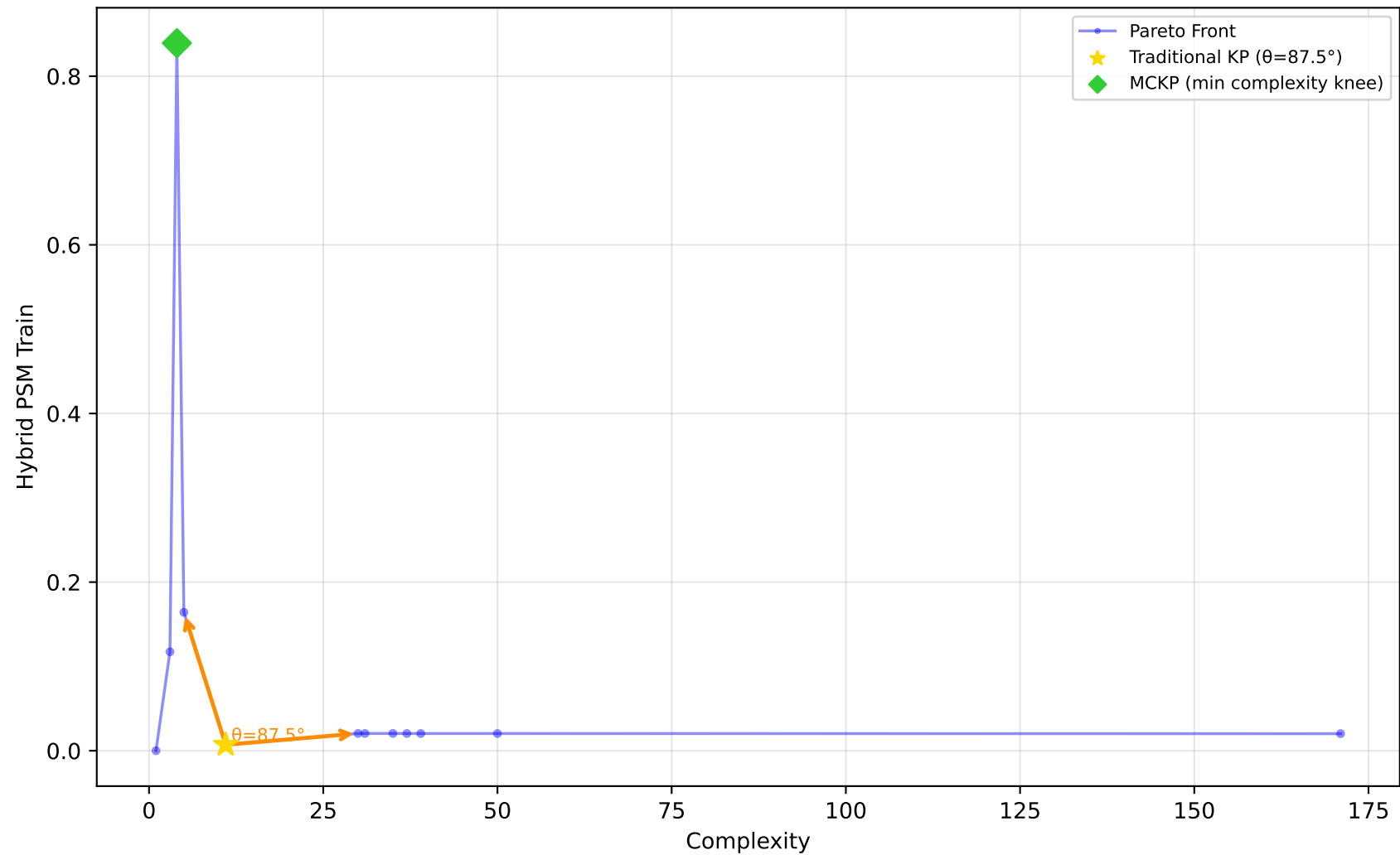
523_analcatdata_neavote - Run 11 - SVP - Hybrid PSM Train \lambda_1=0.00, \lambda_2=0.90, \lambda_3=0.00 | Difficulty: 1.00 | Method: hmr
