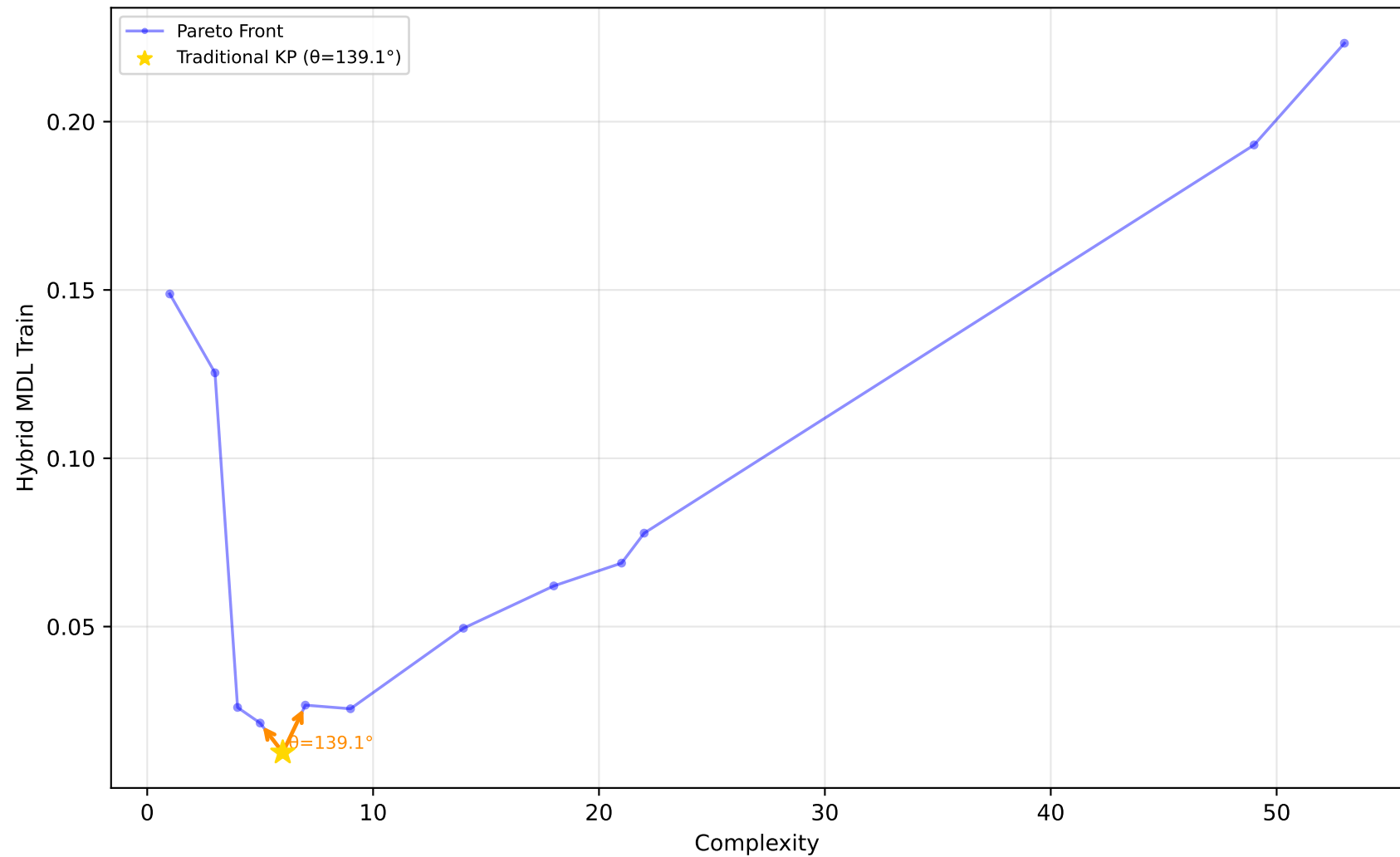
523_analcatdata_neavote - Run 12 - MVP - Hybrid MDL Train \lambda_1=0.00, \lambda_2=0.10, \lambda_3=0.00 | Difficulty: 1.00 | Method: hmr
