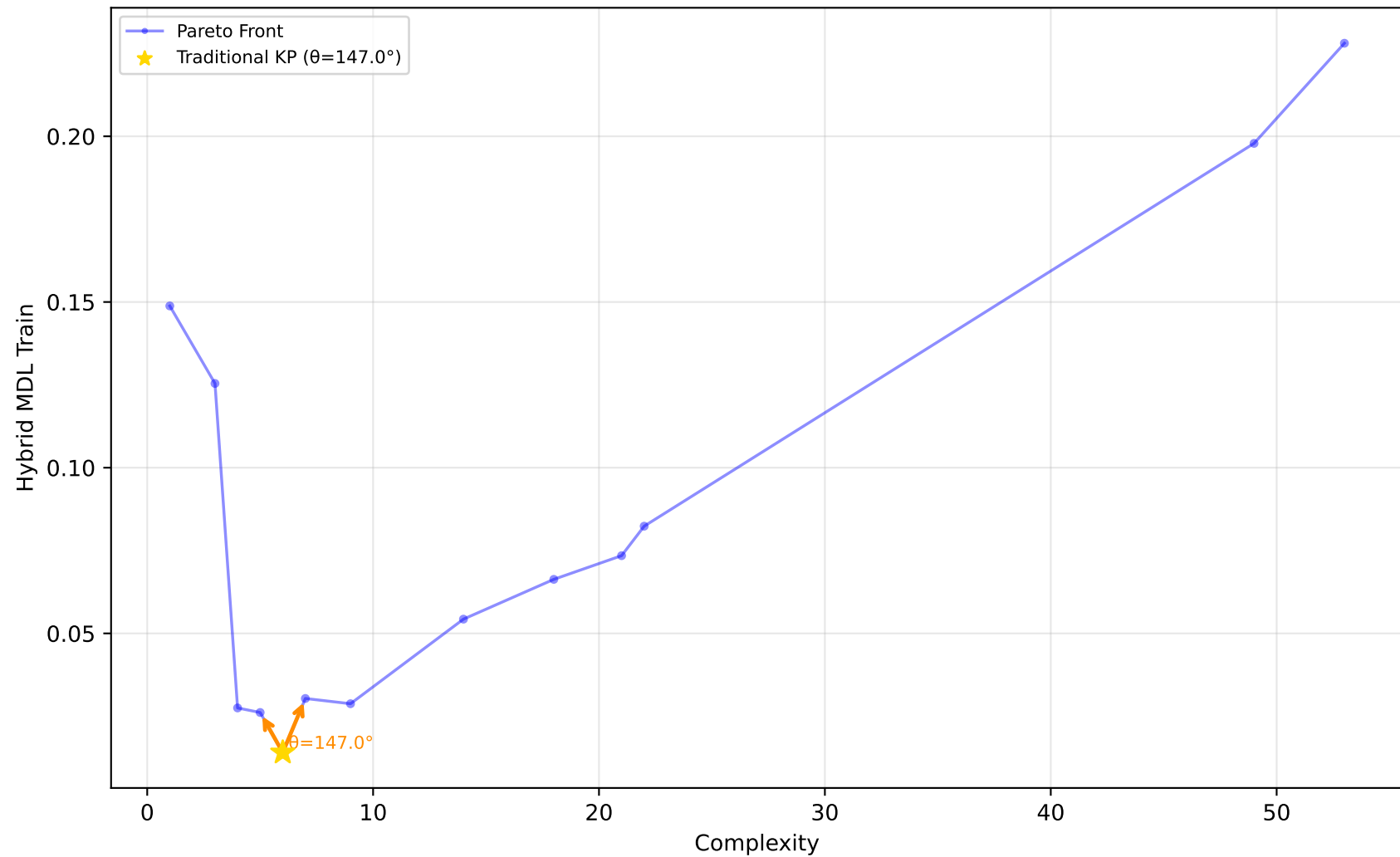
523_analcatdata_neavote - Run 12 - MVP - Hybrid MDL Train \lambda_1=0.00, \lambda_2=0.40, \lambda_3=0.00 | Difficulty: 1.00 | Method: hmr
