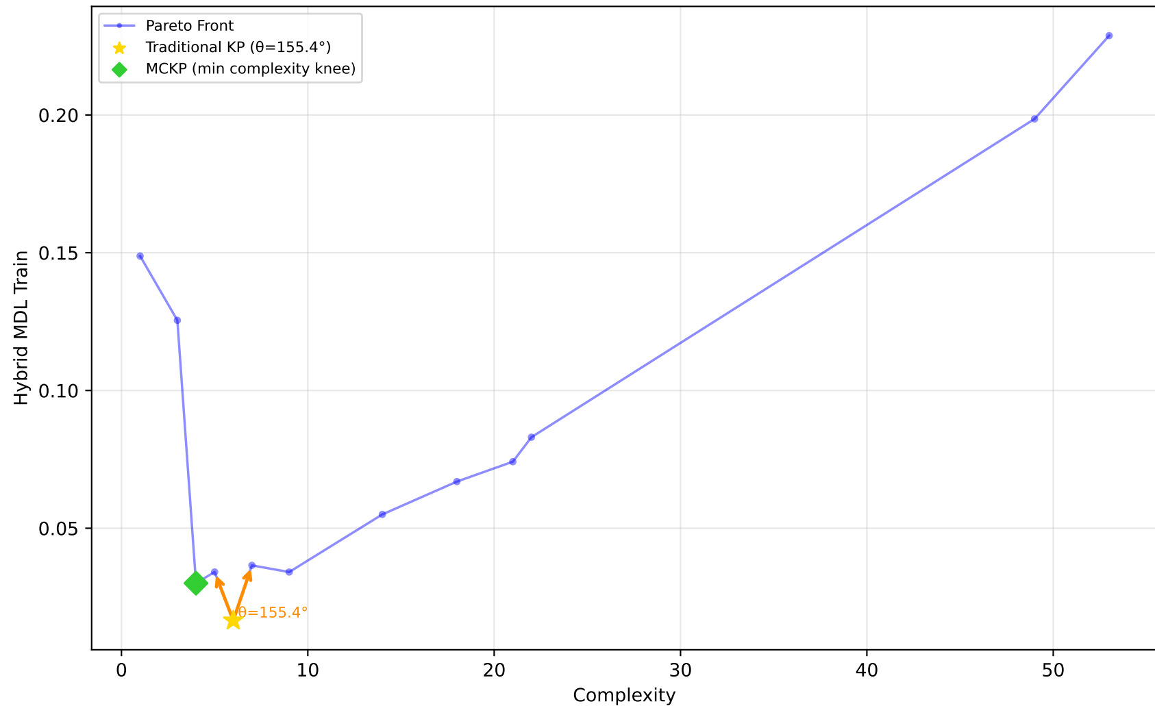
523_analcatdata_neavote - Run 12 - SVP - Hybrid MDL Train \lambda_1=0.00, \lambda_2=0.90, \lambda_3=0.00 | Difficulty: 1.00 | Method: hmr
