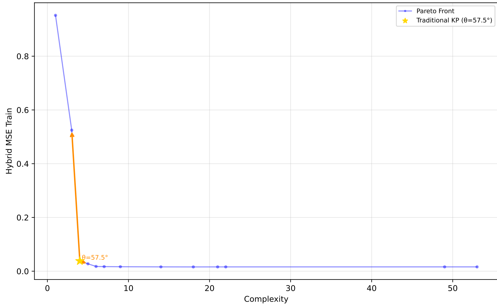
523_analcatdata_neavote - Run 12 - SVP - Hybrid MSE Train \lambda_1=0.00, \lambda_2=0.20, \lambda_3=0.00 | Difficulty: 1.00 | Method: hmr
