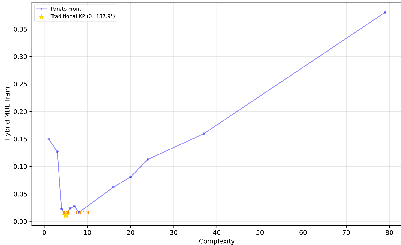
523_analcatdata_neavote - Run 13 - MVP - Hybrid MDL Train \lambda_1=0.00, \lambda_2=0.10, \lambda_3=0.00 | Difficulty: 1.00 | Method: hmr
