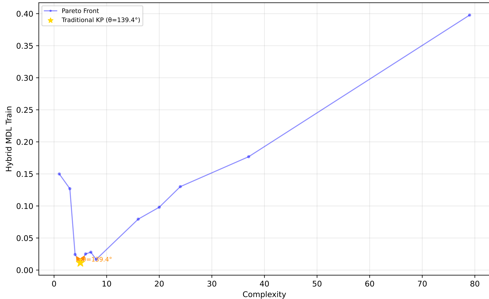
523_analcatdata_neavote - Run 13 - MVP - Hybrid MDL Train \lambda_1=0.00, \lambda_2=0.40, \lambda_3=0.00 | Difficulty: 1.00 | Method: hmr
