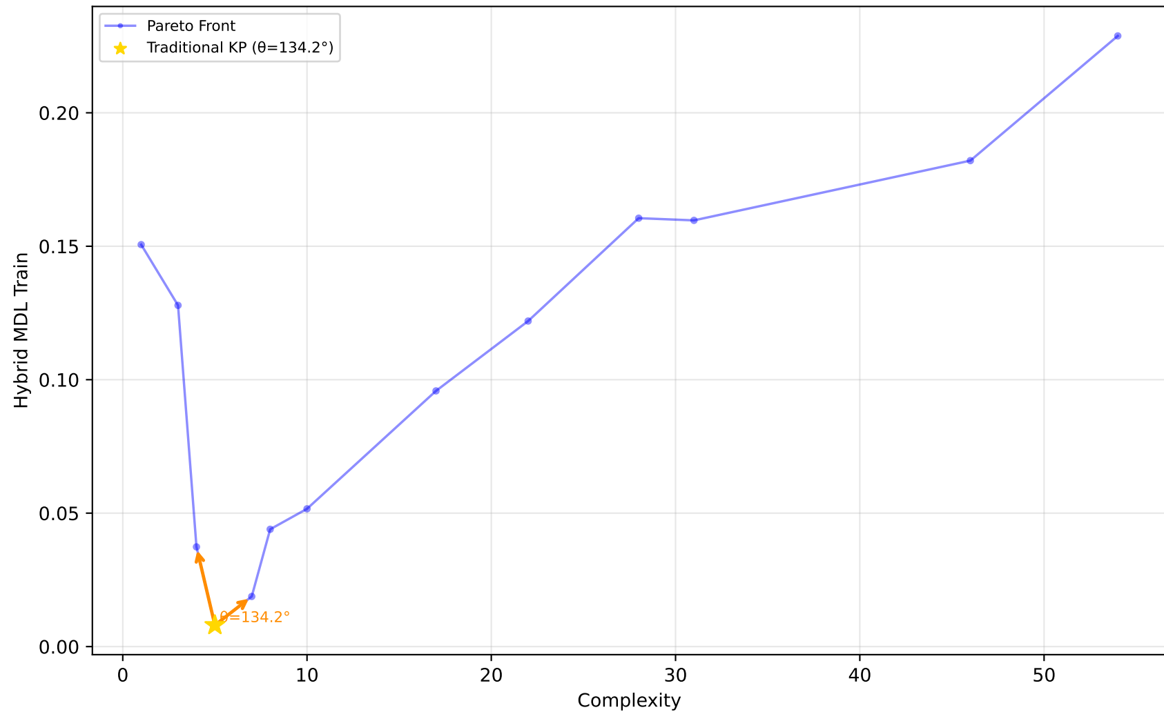
523_analcatdata_neavote - Run 14 - MVP - Hybrid MDL Train \lambda_1=0.00, \lambda_2=0.10, \lambda_3=0.00 | Difficulty: 1.00 | Method: hmr
