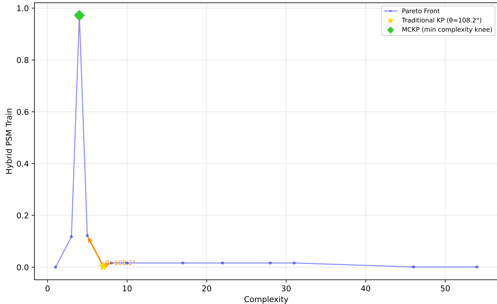
523_analcatdata_neavote - Run 14 - MVP - Hybrid PSM Train \lambda_1=0.00, \lambda_2=0.10, \lambda_3=0.00 | Difficulty: 1.00 | Method: hmr
