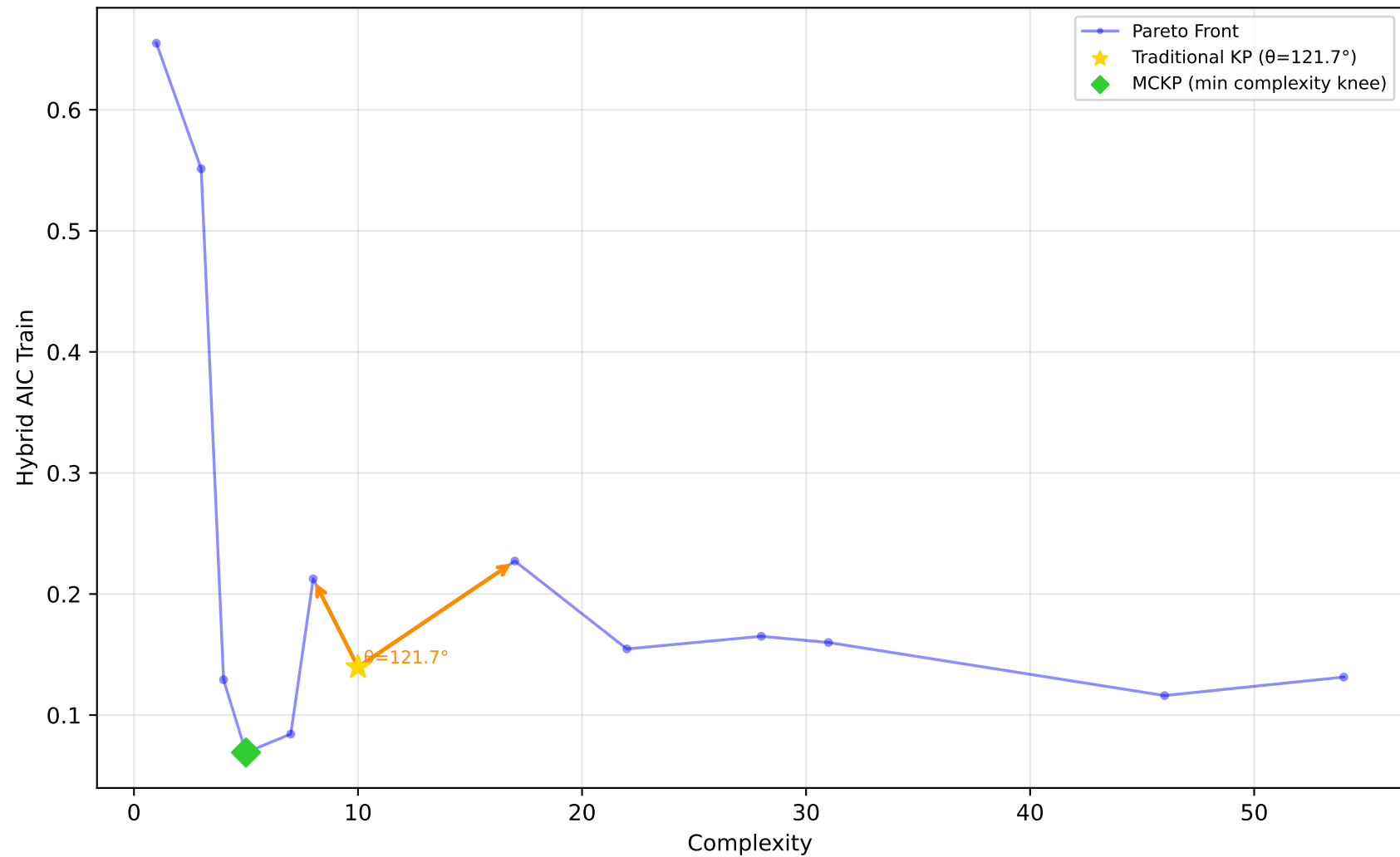
523_analcatdata_neavote - Run 14 - SVP - Hybrid AIC Train \lambda_1=0.00, \lambda_2=0.90, \lambda_3=0.00 | Difficulty: 1.00 | Method: hmr
