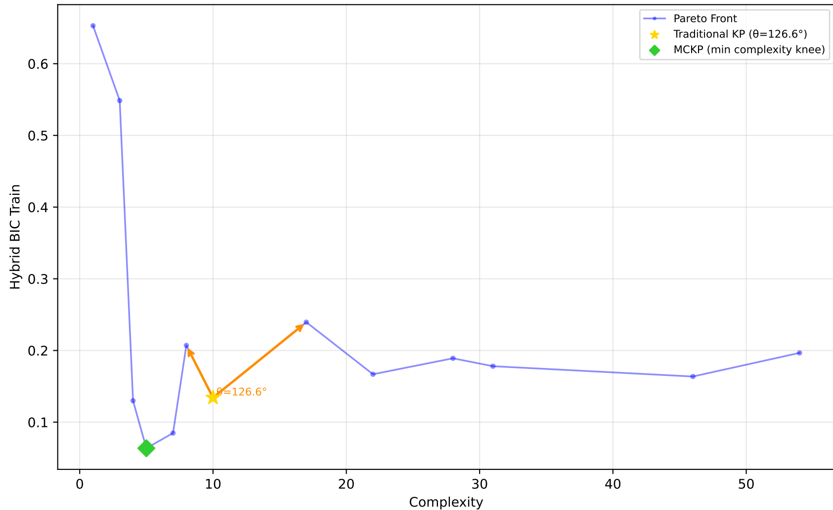
523_analcatdata_neavote - Run 14 - SVP - Hybrid BIC Train \lambda_1=0.00, \lambda_2=0.90, \lambda_3=0.00 | Difficulty: 1.00 | Method: hmr
