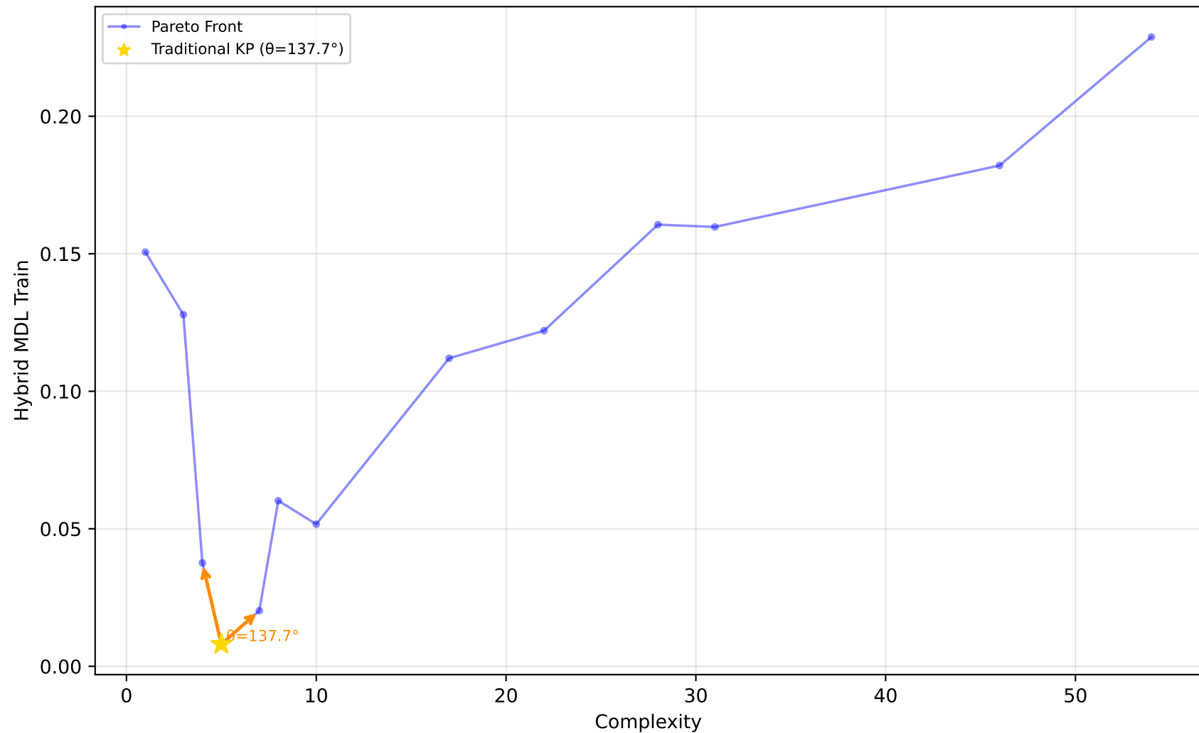
523_analcatdata_neavote - Run 14 - SVP - Hybrid MDL Train \lambda_1=0.00 , \lambda_2=0.20 , \lambda_3=0.00 | Difficulty: 1.00 | Method: hmr
