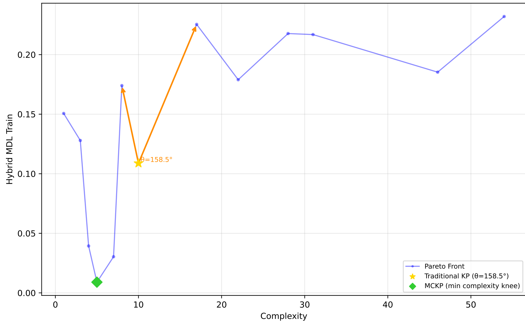
523_analcatdata_neavote - Run 14 - SVP - Hybrid MDL Train \lambda_1=0.00 , \lambda_2=0.90 , \lambda_3=0.00 | Difficulty: 1.00 | Method: hmr
