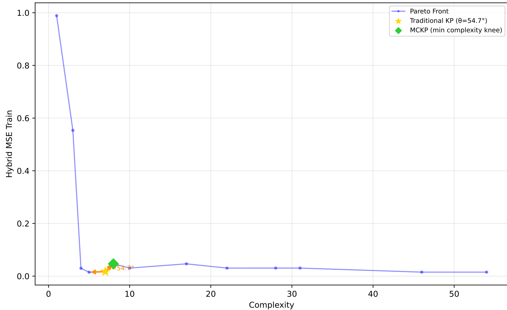
523_analcatdata_neavote - Run 14 - SVP - Hybrid MSE Train \lambda_1=0.00, \lambda_2=0.20, \lambda_3=0.00 | Difficulty: 1.00 | Method: hmr
