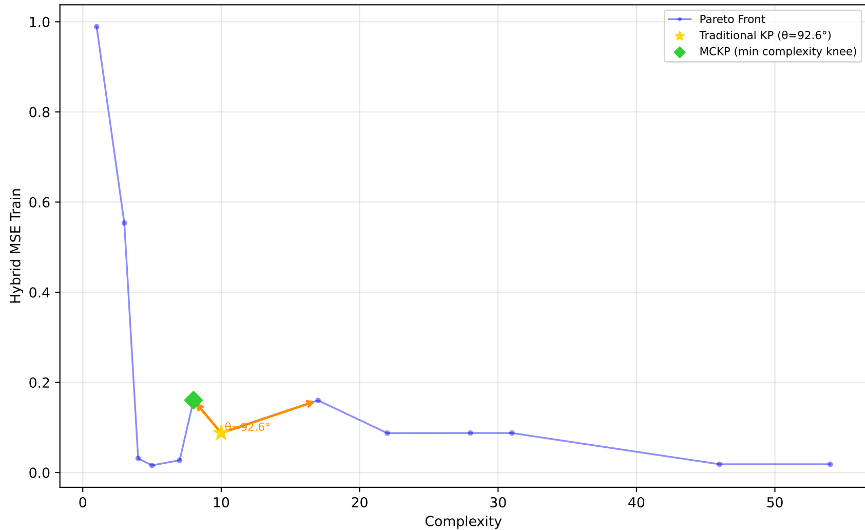
523_analcatdata_neavote - Run 14 - SVP - Hybrid MSE Train \lambda_1=0.00, \lambda_2=0.90, \lambda_3=0.00 | Difficulty: 1.00 | Method: hmr
