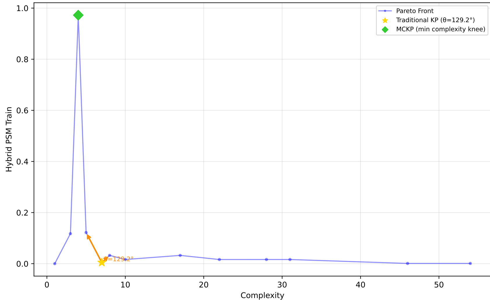
523_analcatdata_neavote - Run 14 - SVP - Hybrid PSM Train \lambda_1=0.00 , \lambda_2=0.20 , \lambda_3=0.00 | Difficulty: 1.00 | Method: hmr
