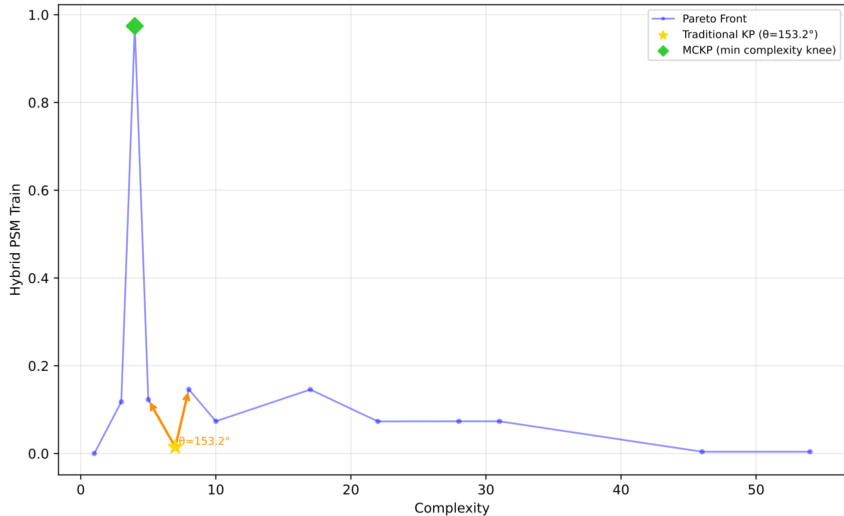
523_analcatdata_neavote - Run 14 - SVP - Hybrid PSM Train \lambda_1=0.00, \lambda_2=0.90, \lambda_3=0.00 | Difficulty: 1.00 | Method: hmr
