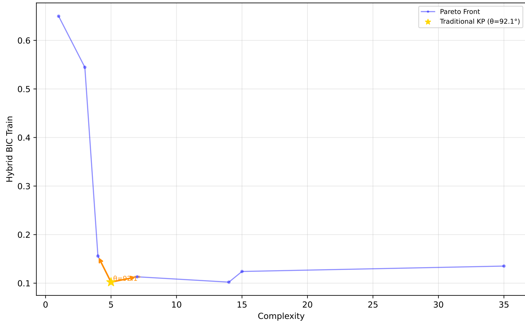
523_analcatdata_neavote - Run 15 - MVP - Hybrid BIC Train \lambda_1=0.00, \lambda_2=0.10, \lambda_3=0.00 | Difficulty: 1.00 | Method: hmr
