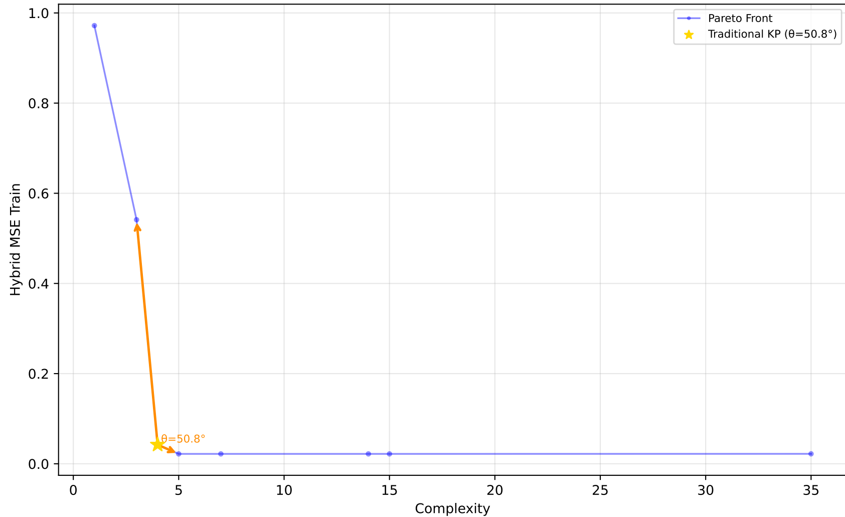
523_analcatdata_neavote - Run 15 - MVP - Hybrid MSE Train \lambda_1=0.00, \lambda_2=0.10, \lambda_3=0.00 | Difficulty: 1.00 | Method: hmr
