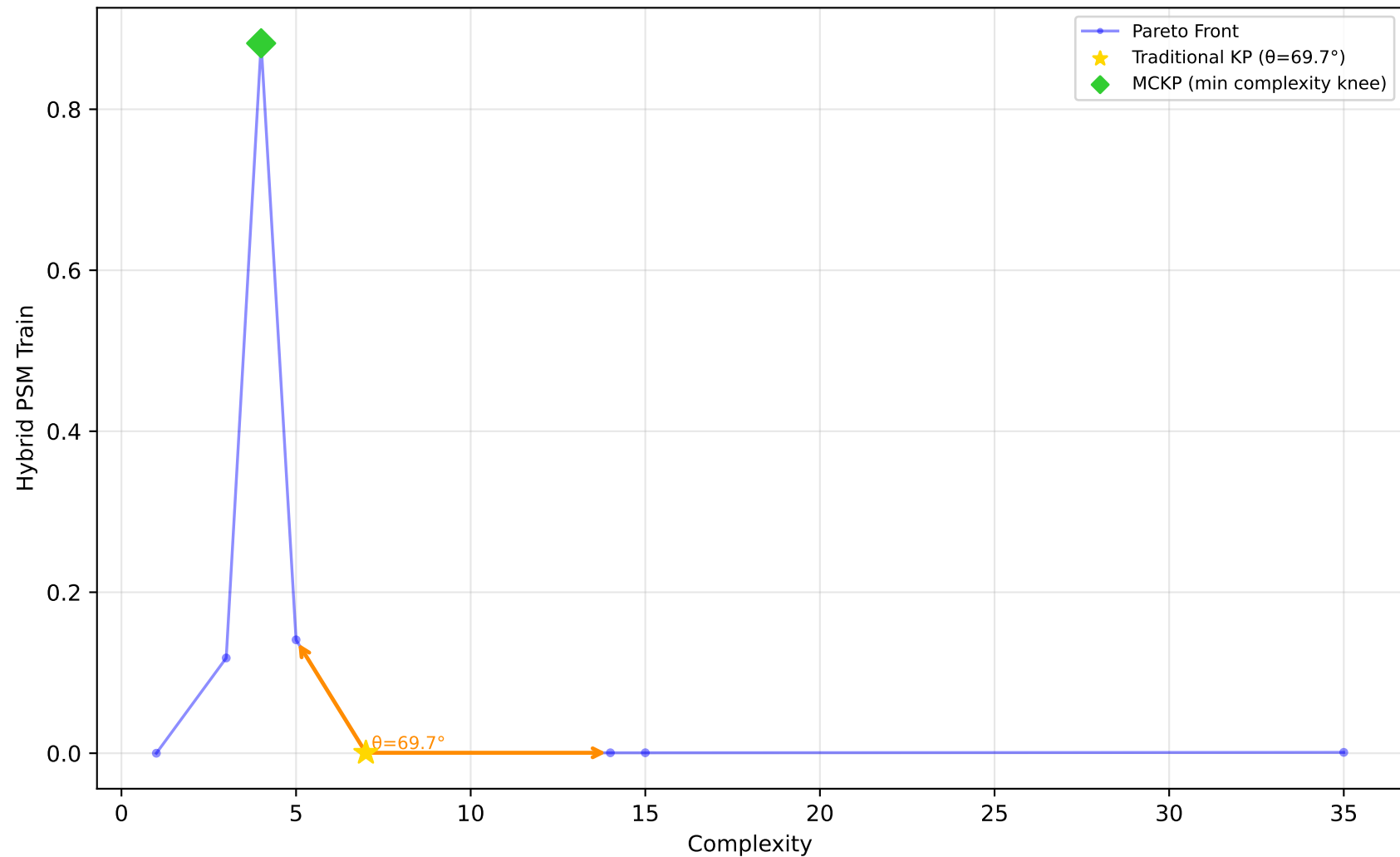
523_analcatdata_neavote - Run 15 - MVP - Hybrid PSM Train \lambda_1=0.00, \lambda_2=0.40, \lambda_3=0.00 | Difficulty: 1.00 | Method: hmr
