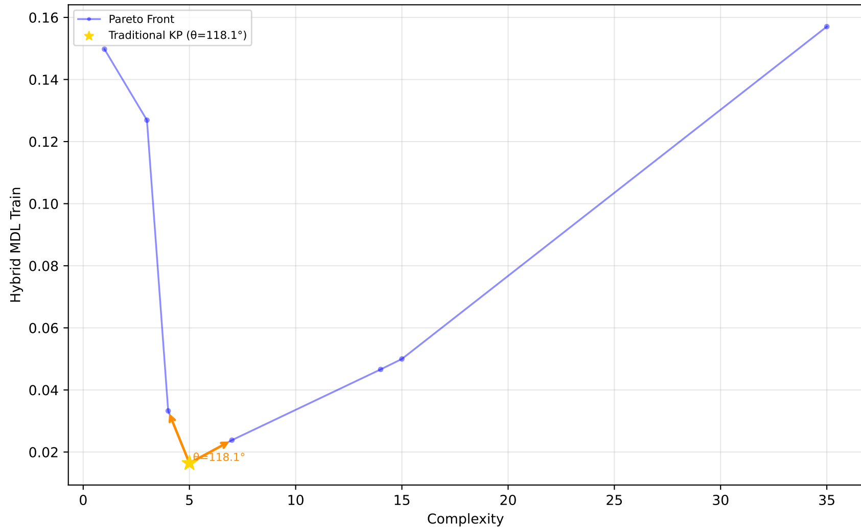
523_analcatdata_neavote - Run 15 - SVP - Hybrid MDL Train \lambda_1=0.00, \lambda_2=0.90, \lambda_3=0.00 | Difficulty: 1.00 | Method: hmr
