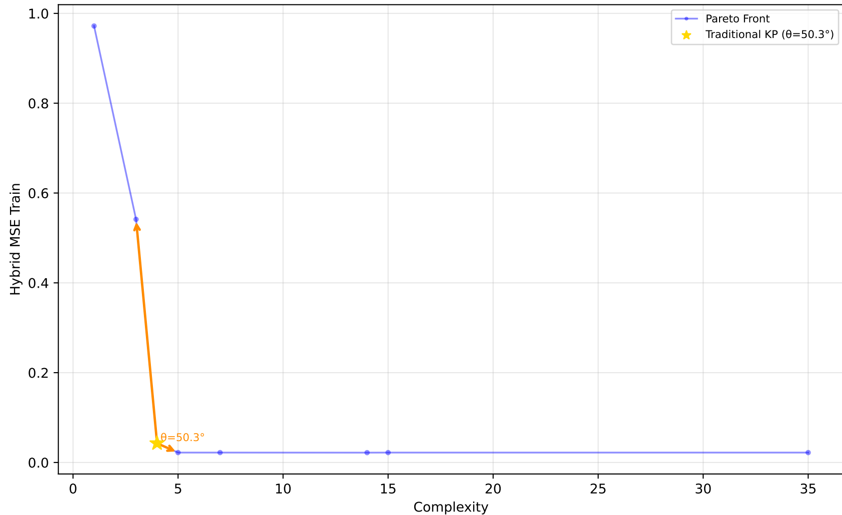
523_analcatdata_neavote - Run 15 - SVP - Hybrid MSE Train \lambda_1=0.00, \lambda_2=0.20, \lambda_3=0.00 | Difficulty: 1.00 | Method: hmr
