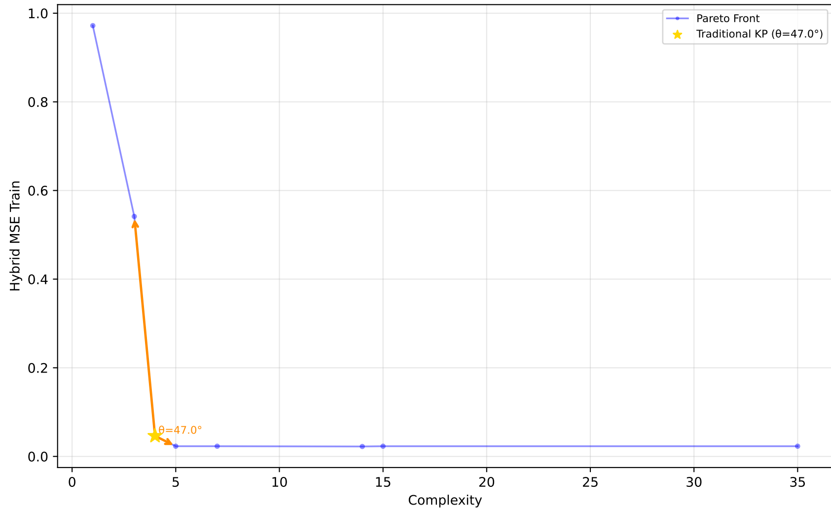
523_analcatdata_neavote - Run 15 - SVP - Hybrid MSE Train \lambda_1=0.00, \lambda_2=0.90, \lambda_3=0.00 | Difficulty: 1.00 | Method: hmr
