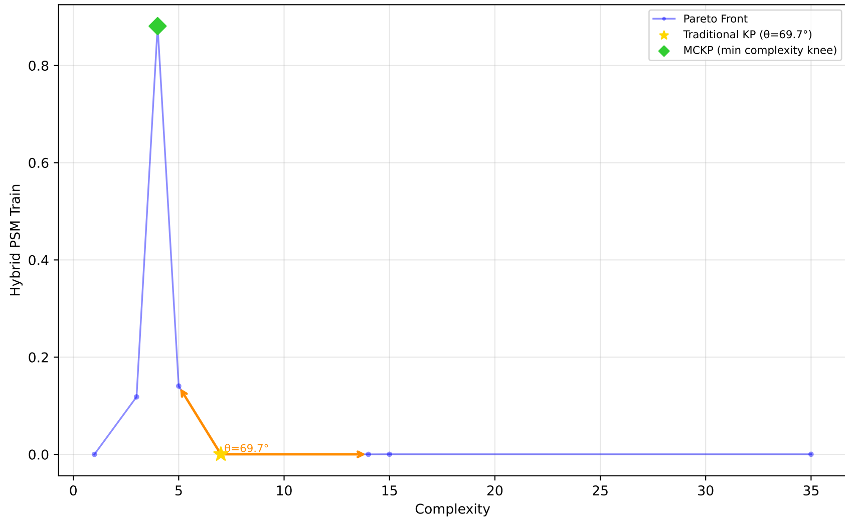
523_analcatdata_neavote - Run 15 - SVP - Hybrid PSM Train \lambda_1=0.00, \lambda_2=0.20, \lambda_3=0.00 | Difficulty: 1.00 | Method: hmr
