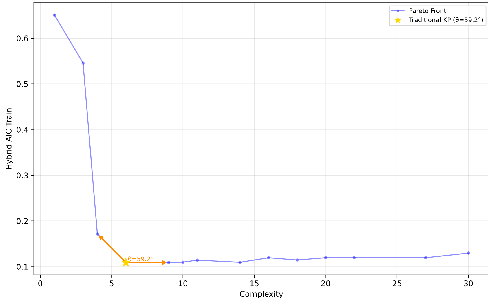
523_analcatdata_neavote - Run 16 - MVP - Hybrid AIC Train \lambda_1=0.00 , \lambda_2=0.10 , \lambda_3=0.00 | Difficulty: 1.00 | Method: hmr
