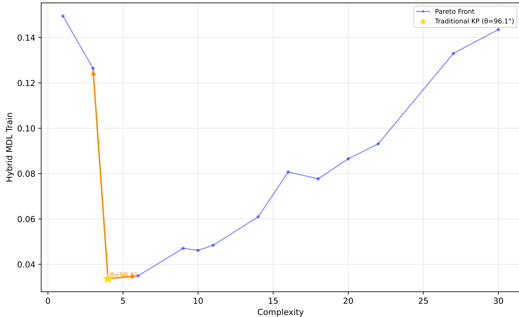
523_analcatdata_neavote - Run 16 - MVP - Hybrid MDL Train \lambda_1=0.00, \lambda_2=0.40, \lambda_3=0.00 | Difficulty: 1.00 | Method: hmr
