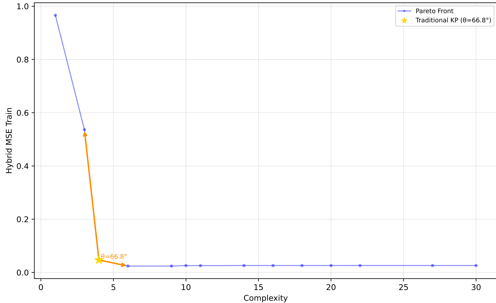
523_analcatdata_neavote - Run 16 - MVP - Hybrid MSE Train \lambda_1=0.00, \lambda_2=0.10, \lambda_3=0.00 | Difficulty: 1.00 | Method: hmr
