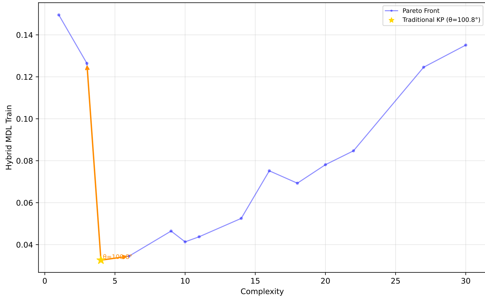
523_analcatdata_neavote - Run 16 - SVP - Hybrid MDL Train \lambda_1=0.00, \lambda_2=0.20, \lambda_3=0.00 | Difficulty: 1.00 | Method: hmr
