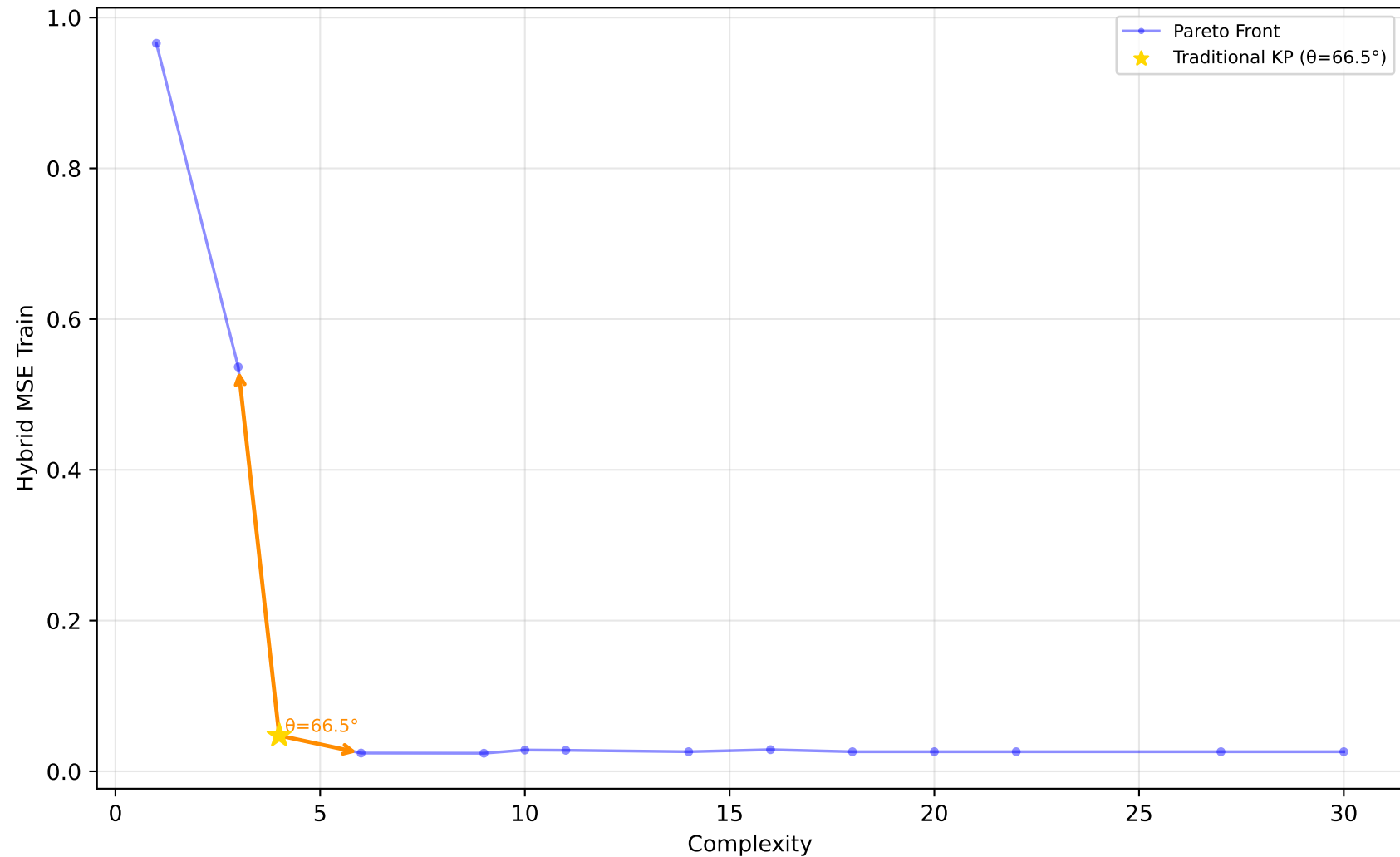
523_analcatdata_neavote - Run 16 - SVP - Hybrid MSE Train \lambda_1=0.00, \lambda_2=0.20, \lambda_3=0.00 | Difficulty: 1.00 | Method: hmr
