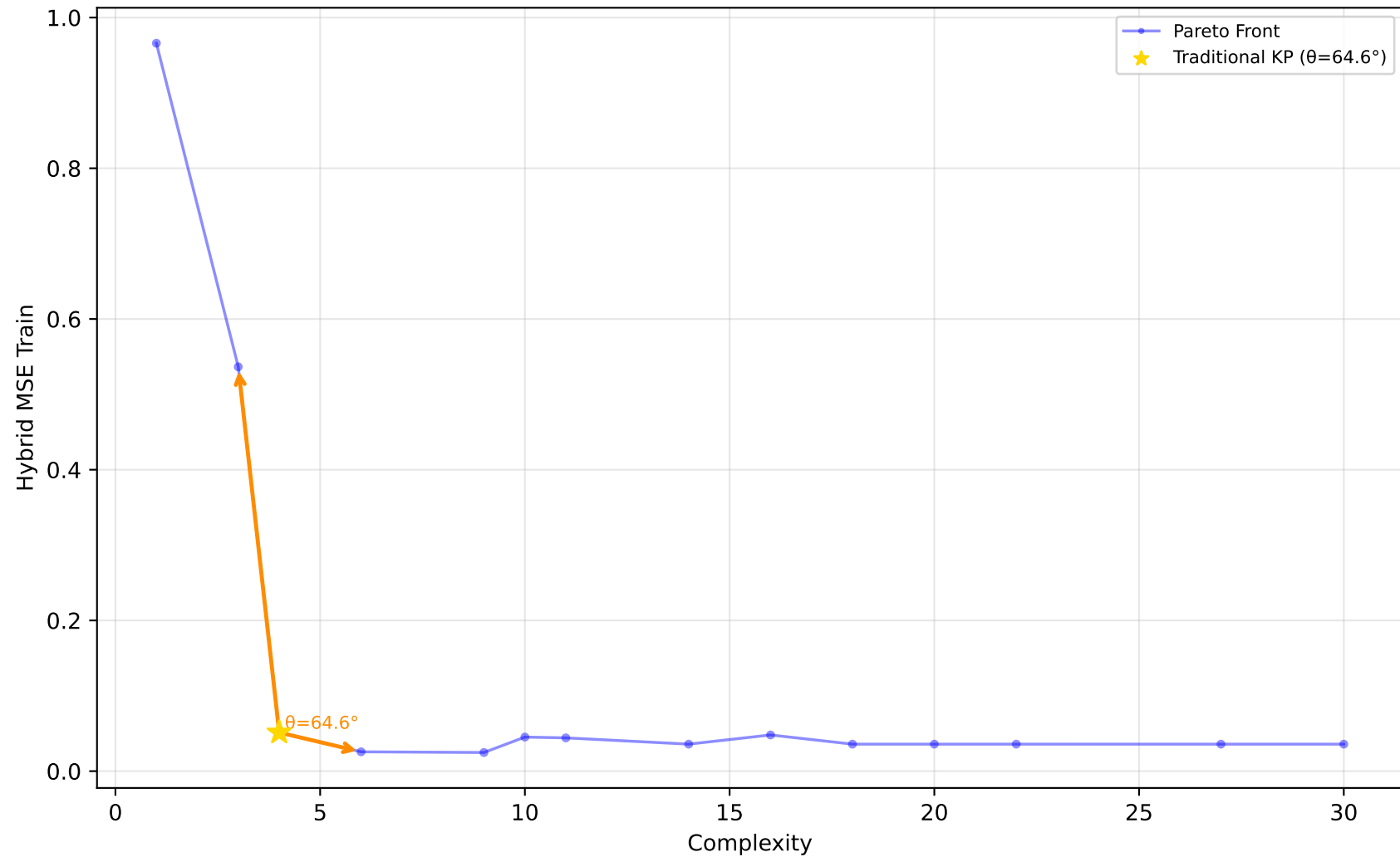
523_analcatdata_neavote - Run 16 - SVP - Hybrid MSE Train \lambda_1=0.00, \lambda_2=0.90, \lambda_3=0.00 | Difficulty: 1.00 | Method: hmr
