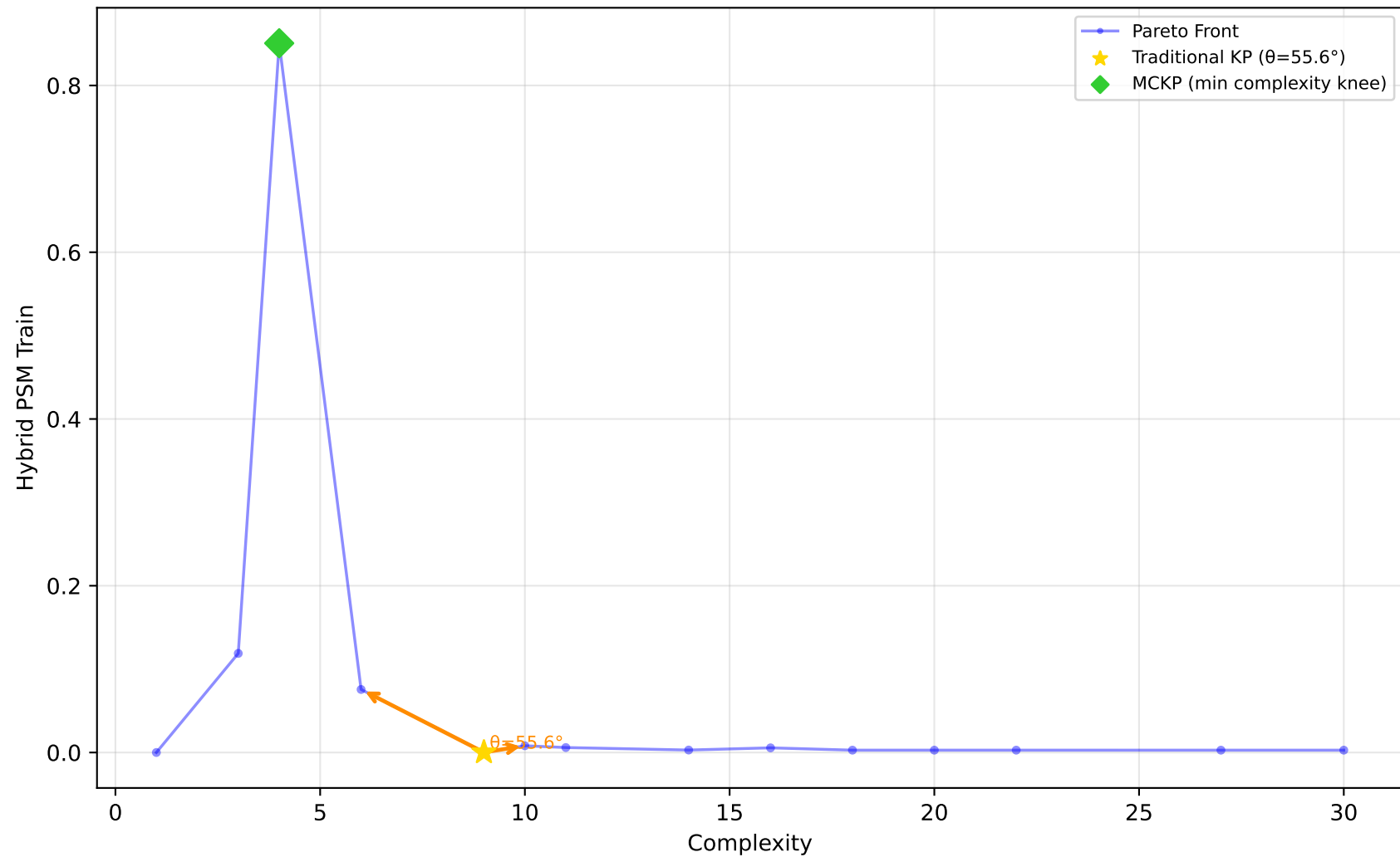
523_analcatdata_neavote - Run 16 - SVP - Hybrid PSM Train \lambda_1=0.00 , \lambda_2=0.20 , \lambda_3=0.00 | Difficulty: 1.00 | Method: hmr
