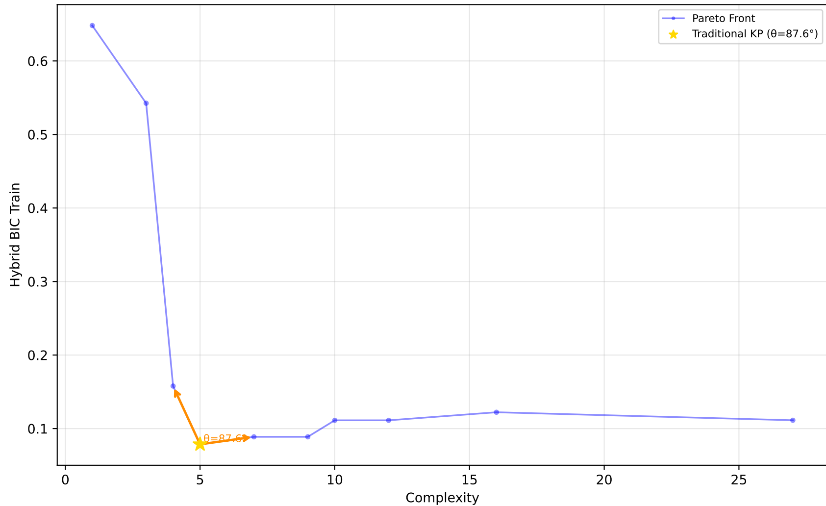
523_analcatdata_neavote - Run 17 - MVP - Hybrid BIC Train \lambda_1=0.00, \lambda_2=0.10, \lambda_3=0.00 | Difficulty: 1.00 | Method: hmr
