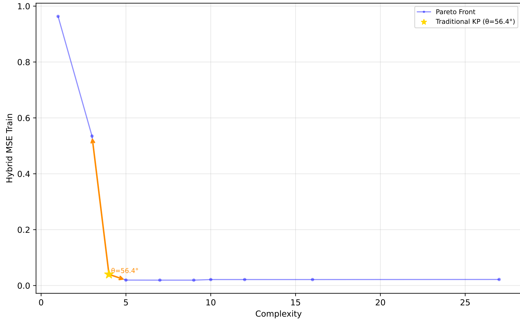
523_analcatdata_neavote - Run 17 - MVP - Hybrid MSE Train \lambda_1=0.00, \lambda_2=0.40, \lambda_3=0.00 | Difficulty: 1.00 | Method: hmr
