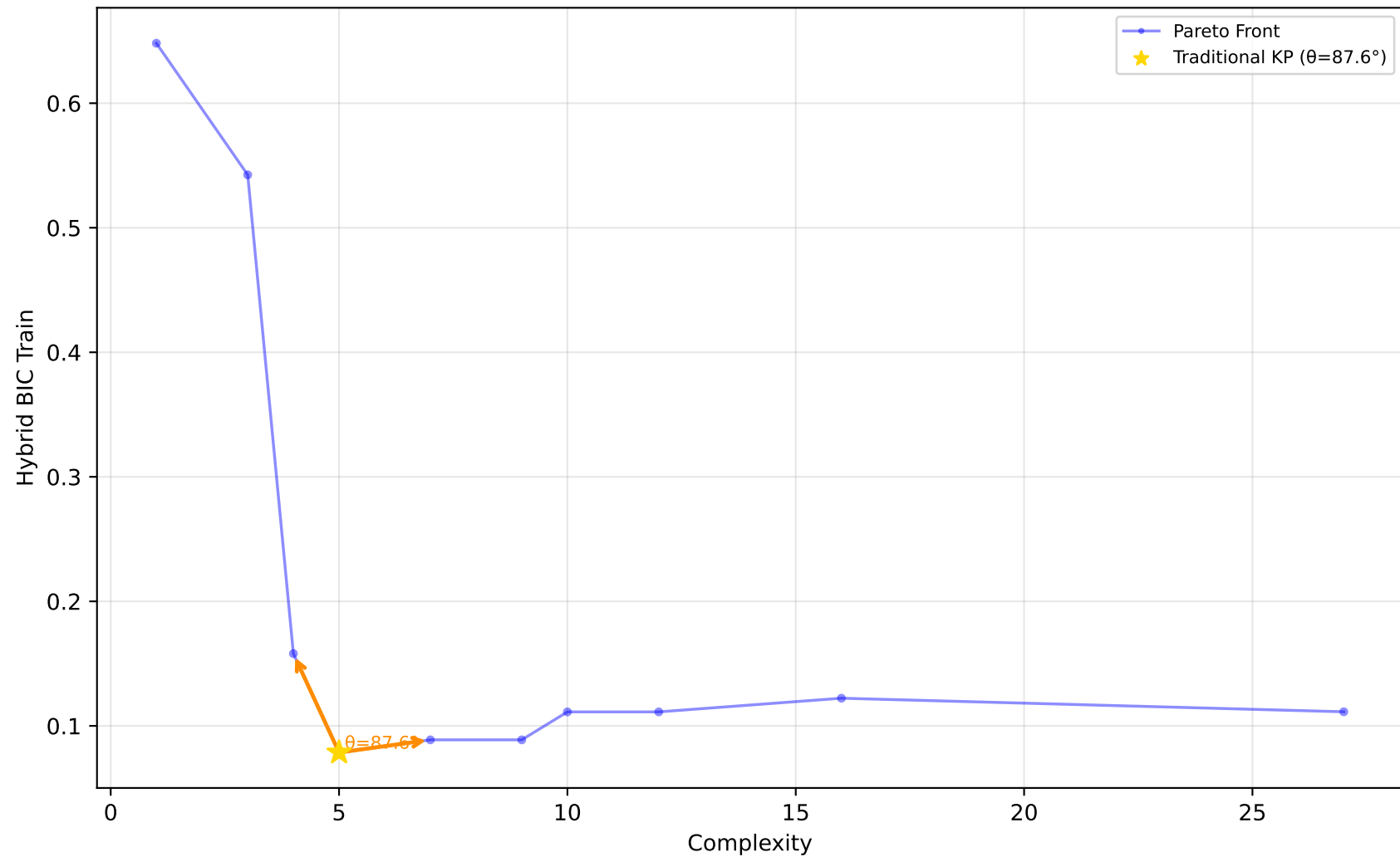
523_analcatdata_neavote - Run 17 - SVP - Hybrid BIC Train \lambda_1=0.00 , \lambda_2=0.20 , \lambda_3=0.00 | Difficulty: 1.00 | Method: hmr
